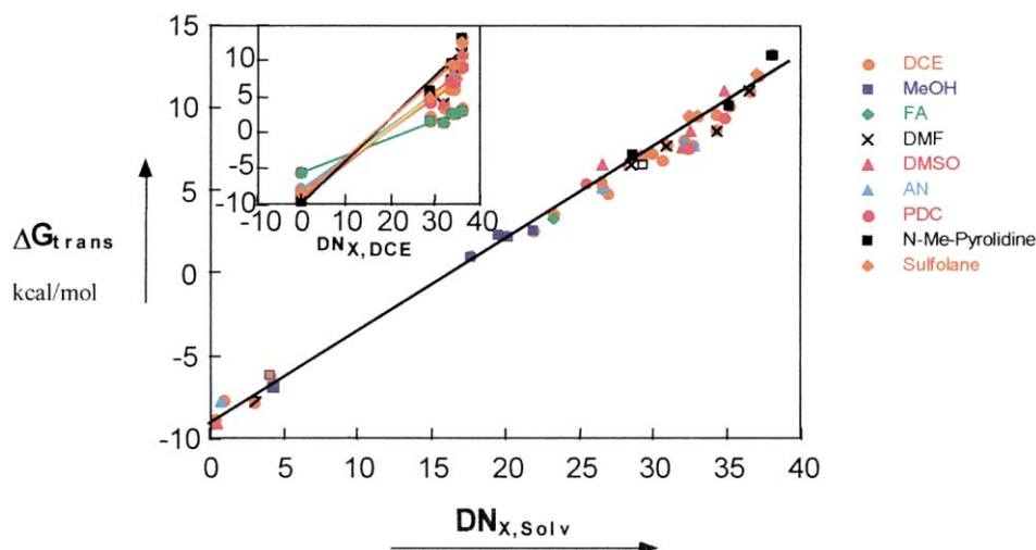
Fig. 17. Free energies of transfer ( \Delta G_{\text{trans}} ) of various anions ( \text{B}\phi_4^- , \text{I}^- , \text{Br}^- , \text{SCN}^- , \text{Cl}^- ) from water to various solvents versus the donor number of the anion in 1,2-dichloroethane ( \text{DN}_{\text{X,DCE}} ), given in the insert, and versus the donor number of the anion in the respective solvent \text{DN}_{\text{X,Solv}} [4] (reproduced by permission of The Royal Society of Chemistry).
