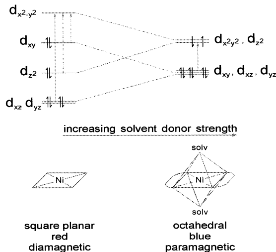
Fig. 4. Solvatochromism and thermochromism of [\text{Ni}(\text{dike})(\text{diam})]^+ complexes are due to a change from square-planar to octahedral coordination. In the case of the Ni(II) system ( d^8 ) this leads, besides the spectral changes, to a change in the magnetic behaviour from diamagnetic to paramagnetic species [37,10] (with permission from Research Trends).
