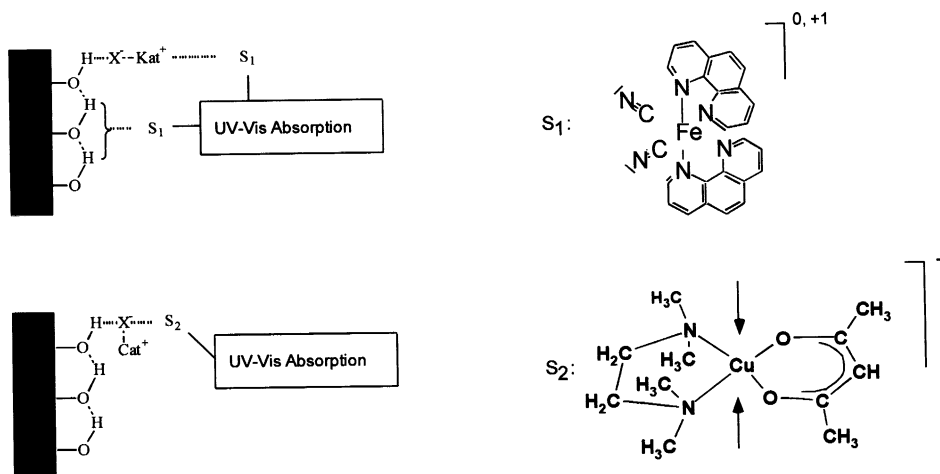
Fig. 23. Estimation of donor and acceptor properties of active surfaces and their interaction with cations and anions by means of solvatochromic indicators (kindly supplied by S. Spange).
