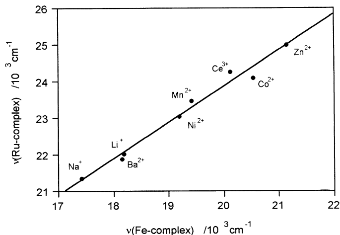
Fig. 21. Absorption maxima in the spectra of \text{Ru}(\text{phen})_2(\text{CN})_2 versus those in the spectra of \text{Fe}(\text{phen})_2(\text{CN})_2 in the presence of different cations in acetonitrile. \nu_{\text{Ru}} = 0.991 \nu_{\text{Fe}} + 4040 ( r = 0.991 ) [23] (with permission from Gordon and Breach Publishers).
