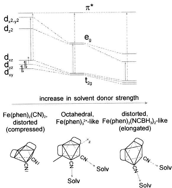
Fig. 15. Solvatochromism of \text{Fe}(\text{phen})_2(\text{CN})_2 and [\text{Fe}(\text{phen})_2(\text{CN})_2]^+ [52]. (used with permission from the Journal of Chemical Education, vol. 62, no. 6, 1985, pp. 459–462; ©copyright 1985, Division of Chemical Education, Inc.).
