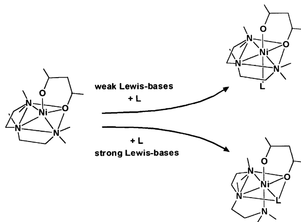
Fig. 6. Structural variation of the five-coordinated mixed-ligand Ni(II) complex [\text{Ni}(\square\text{-dike})(\text{pmdt})]^+ interacting with donor molecules of different Lewis basicity [10] ( \beta\text{-dike} ).
