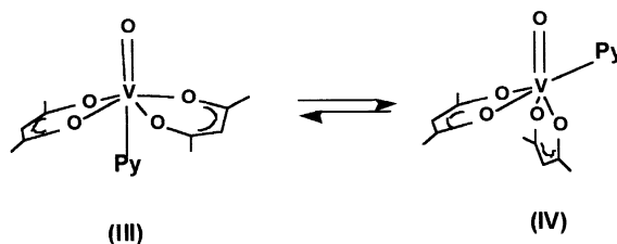
Fig. 11. Structural variability of \text{VO}(\text{acac})_2\text{Py} .
