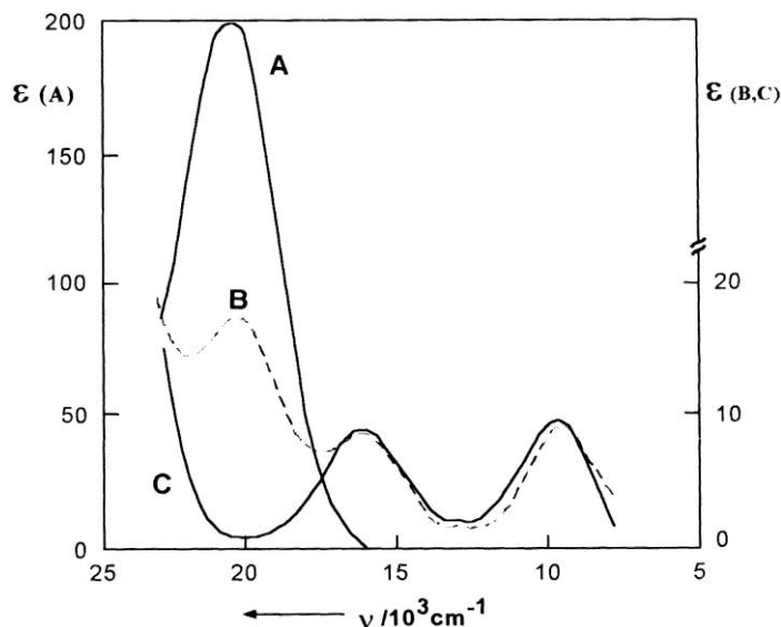
Fig. 3. UV-vis absorption spectra of [\text{Ni}(\text{acac})(\text{tmen})]\text{BPh}_4 in: (A) DCE; (b) acetone; and (C) DMF at 25°C [15] (with permission from Springer Verlag and authors).
