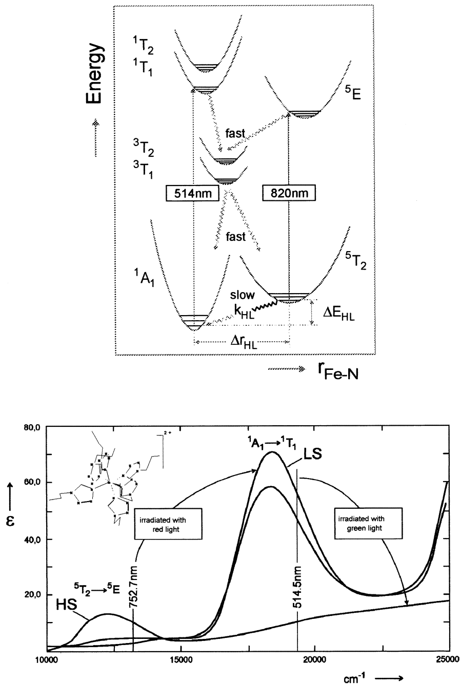
Fig. 28. LIESST effect of Fe(ptz)_6(BF_4)_2 at 10 K (ptz = 1- n -propyltetrazole). Fe(ptz)_6(BF_4)_2 a spin-crossover compound exhibiting strongly pronounced, sharp thermally and optically excited spin transitions. The spin-crossover is visualised by a colour change from white (HS) to violet (LS) occurring around 130 K. Green light changes low-spin states to high-spin states. Red light reverses this process [41] (with permission from Springer Verlag and authors).
